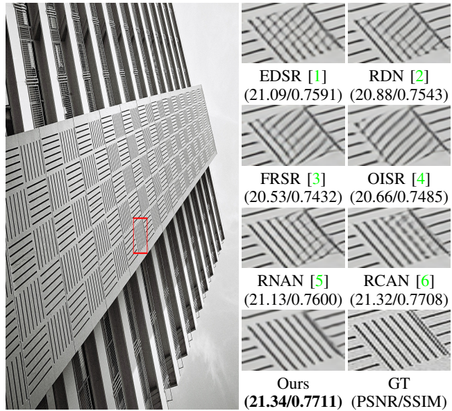
Fig. 1. Visual comparison between different algorithms on img092 from Urban100 [7] with scale factor \times 3 . Our TSAN obtains better visual quality and recovers more image details compared with other state-of-the-art SR methods.
